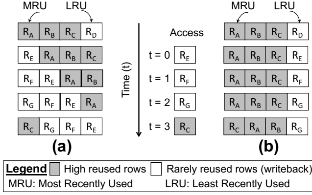
Fig. 6. Example illustrating (a) Traditional LRU policy (b) Our Row Buffer Management policy
