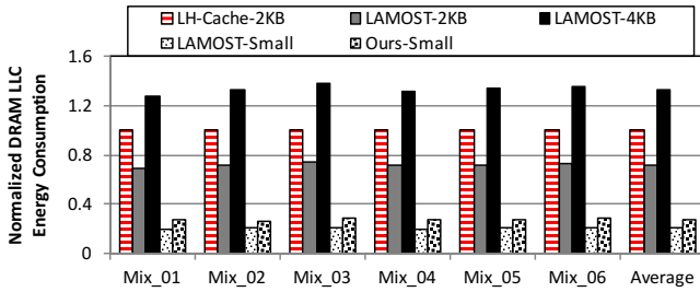
Fig. 11. Energy comparison of our proposed organization compared to state-of-the-art approaches
