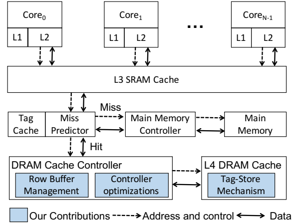
Fig. 1. Typical DRAM based multi-core cache hierarchy for an N-core system; see Section IV-A and Table III for core and cache parameters
