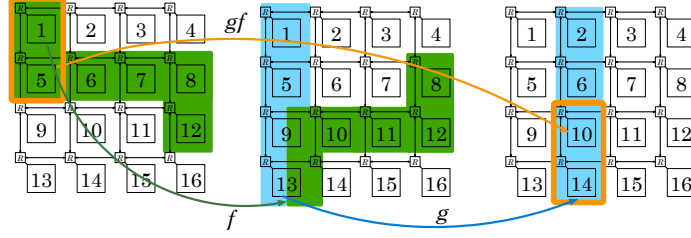
Figure 6: The product of partial permutations.
