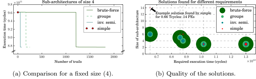
Figure 17: Comparison of strategies for resource-constrained mapping.
