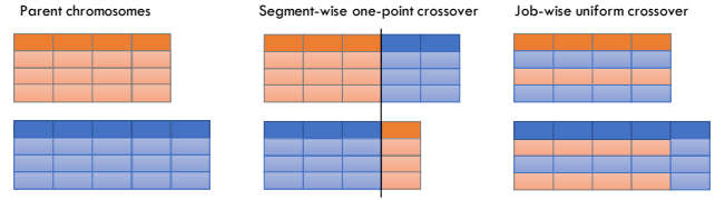
Fig. 3. Crossover operators applied to parent individuals (left): segment-wise one-point (center) and job-wise uniform (right).
