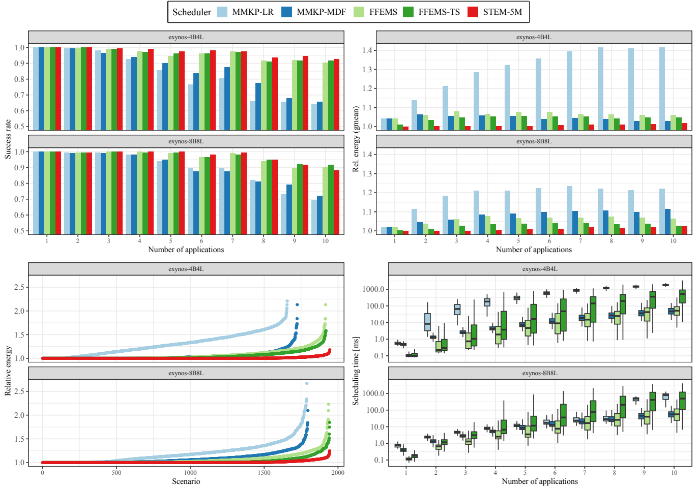
Fig. 4. Performance comparison of schedulers across two heterogeneous platforms concerning success rate (top left), relative energy consumption (top right), and scheduling time (bottom right). The bottom left plot showcases the monotonic curves of the relative energies.
