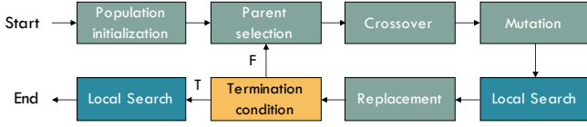
Fig. 2. The STEM algorithm flow.
