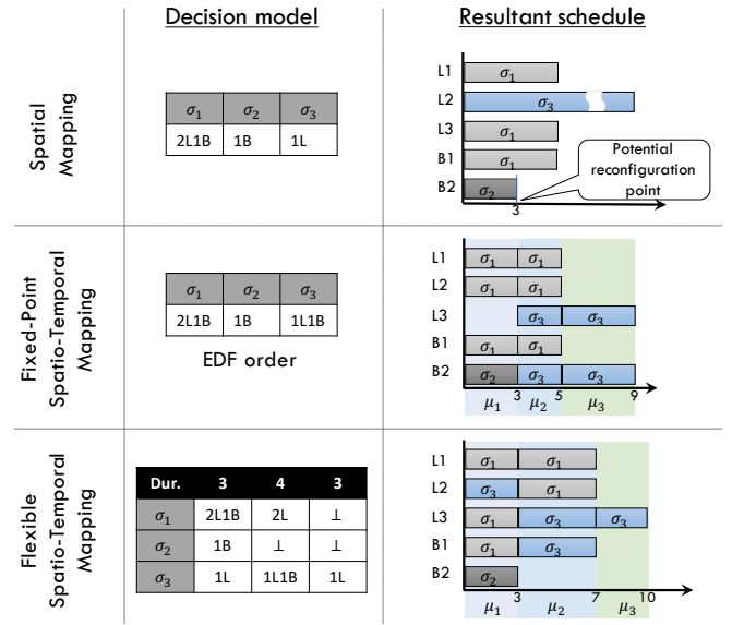
Fig. 1. Overview of multi-application mapping models. Spatial mapping selects one configuration per application, ensuring simultaneous selection. Fixed-point spatio-temporal mapping also picks one configuration per application and, with a specified application order, finalizes a spatio-temporal mapping. Flexible spatio-temporal mapping designates mapping segments and their durations, ensuring all specified configurations (with \perp denoting idle) within the segment can coexist.
