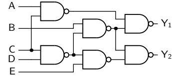
Fig. 3. C17 benchmark circuit [25] in NAND configuration
