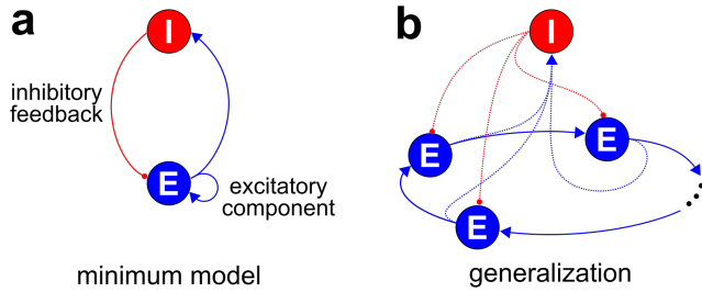
FIGURE 1. Spiking neural circuit motifs that implement a 1-bit volatile memory. Blue circles labeled as ‘E’ represent excitatory neurons, red circles labeled as ‘I’ represent inhibitory neurons, circles as arrow heads represent inhibitory connections and conventional arrows represent excitatory connections. (a) A minimal circuit composed of two neurons, one excitatory and one inhibitory. (b) A circuit composed of an excitatory ring sub-network and an inhibitory neuron. (a-b) In both cases, the excitatory component has self-connections and connections to the inhibitory neurons while the inhibitory feedback connects to all excitatory neurons.
